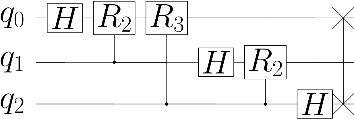
This figure was created using Qiskit (Javadi-Abhari et al. 2024) and verified using NVIDIA's CUDA-Q v13.2 (NVIDIA 2026), applying a comparison against the QFT matrix that we apply on |000\rangle to obtain our expected result (Qiskit and CUDA-Q are Python packages).
