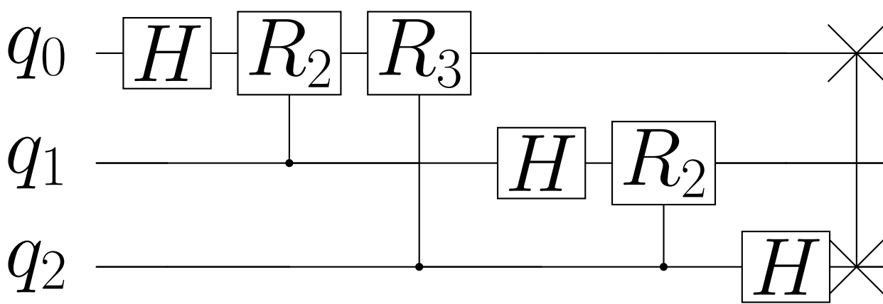
This figure was created using Qiskit (Javadi-Abhari et al. 2024) and verified using NVIDIA's CUDA-Q v13.2 (NVIDIA 2026), applying a comparison against the QFT matrix that we apply on |000⟩ to obtain our expected result (Qiskit and CUDA-Q are Python packages).
