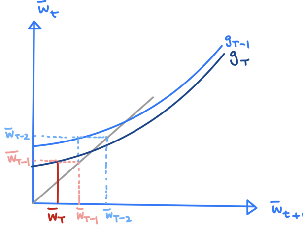
Figure 3.1: Using induction to show \bar{w}_t < \bar{w}_{t+1}
