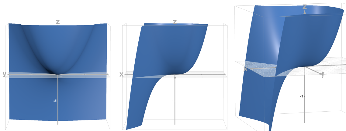
Figure 1.2.1: A function that is not transversal at the origin
