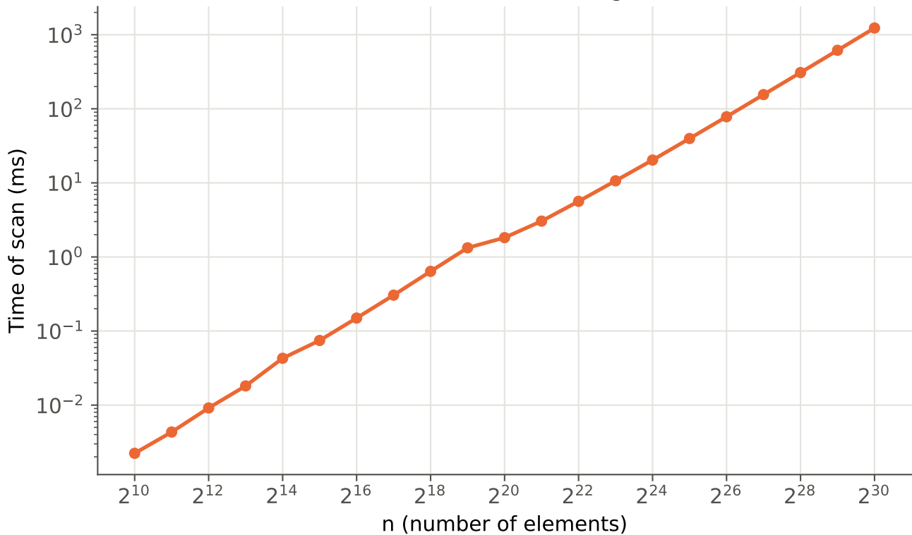
task1: inclusive scan scaling on Euler
