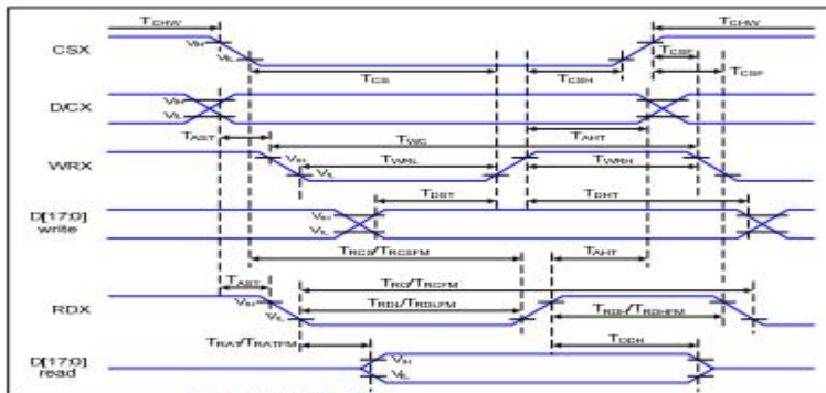
Figure 1 Parallel Interface Timing Characteristics (8080-Series MCU Interface)
