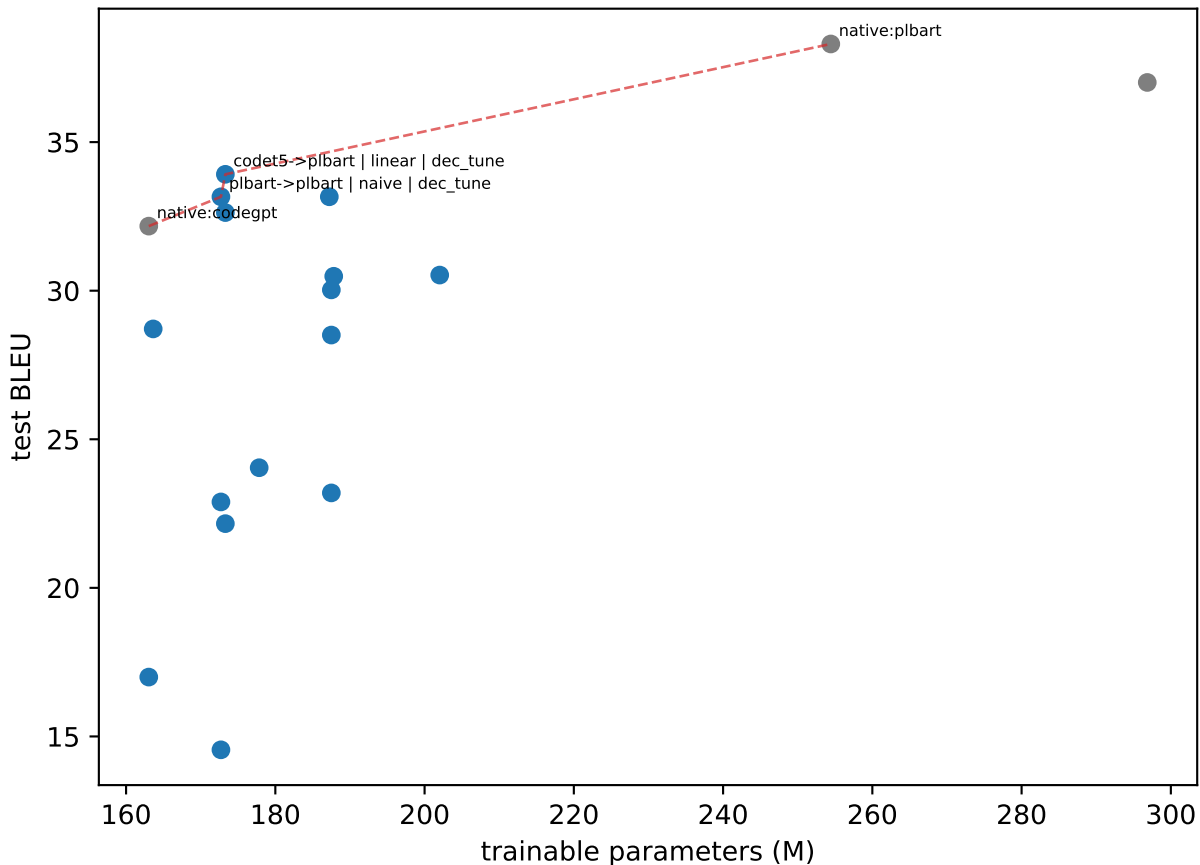
quality vs. trainable-parameter cost (dashed = Pareto frontier)
