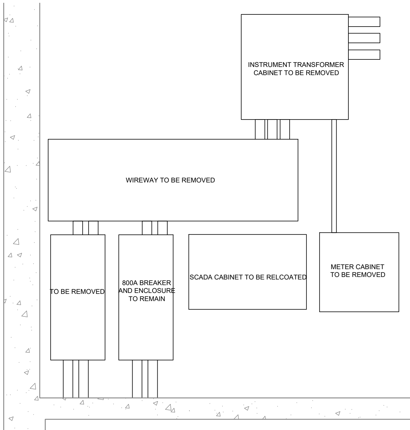
EXISTING ELECTRICAL SERVICE ENTRANCE
