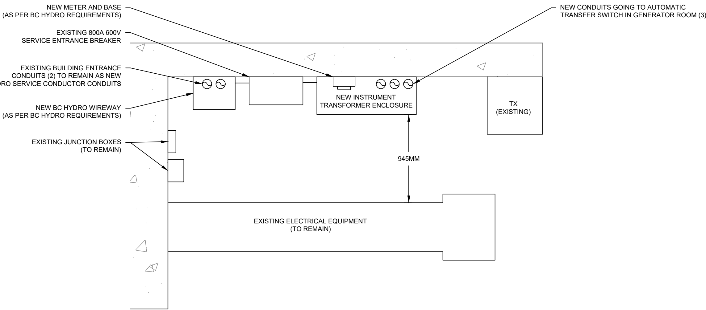
PROPOSED ELECTRICAL SERVICE ENTRANCE - PLAN VIEW
