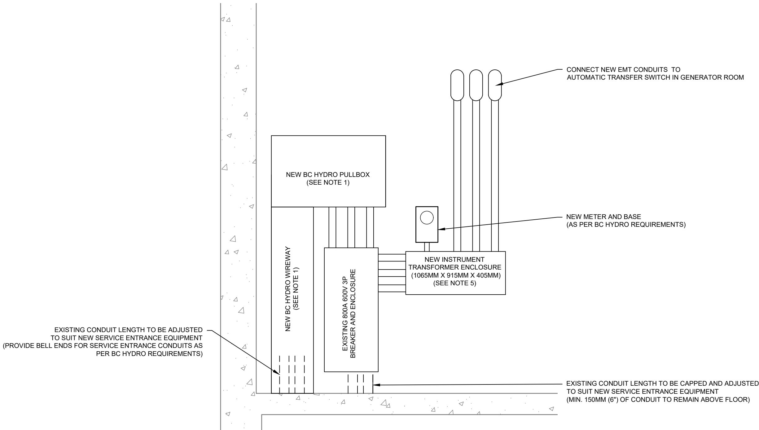
PROPOSED ELECTRICAL SERVICE ENTRANCE SECTIONAL VIEW
