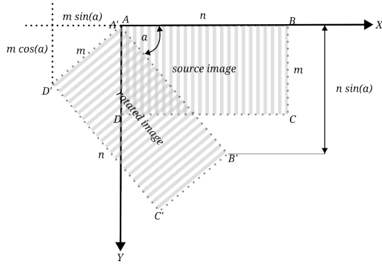
Fig. 1: Example demonstrating rotation of an image in the column major. Thus, every column vector of pixels are rotated at once (Represented by the strips in the image).
