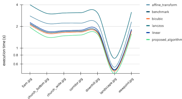
Fig. 8: Algorithm Performance Across Various Images (scale is logarithmic)
