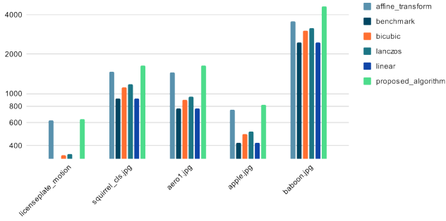
Fig. 5: LMSE analysis (scale is logarithmic)
