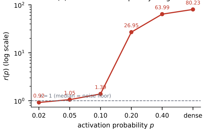
(b) drift across the sparsity range
