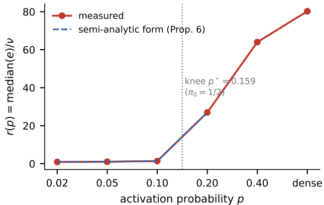
(a) reference-scale ratio
