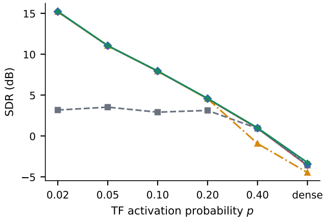
(b) end-to-end source quality
