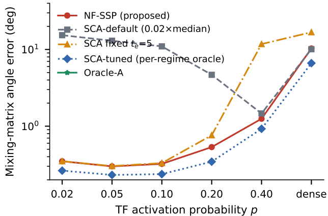
(a) mixing-matrix accuracy
