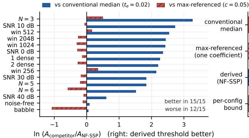
(a) Paired comparison, 15 real-speech configurations
