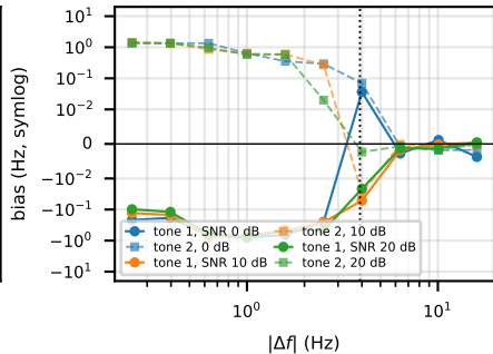
(c) per-tone bias, \rho = 0 dB
