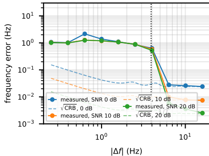
(a) RMSE vs \sqrt{\text{CRB}} , \rho = 0 dB
