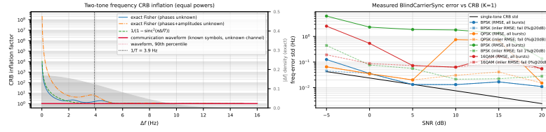
Fig. 2. Left: exact two-tone frequency-CRB inflation vs. offset for the carrier-only surrogate, phases the only nuisance parameters (solid), resp. gains also unknown (dash-dotted); the known-symbol communication-waveform Fisher matrix (Remark 1) shows no coupling (red, near-flat at 1 \times ); sinc 2 heuristic (dashed), 1/T_{\text{burst}} (dotted), benchmark |\Delta f| density (shaded, right axis). Right: measured BlindCarrierSync error vs. single-tone CRB on K=1 bursts: all-burst RMSE (solid) and inlier RMSE (dashed; failures |f - f| > 1 Hz excluded, rates in legend).
