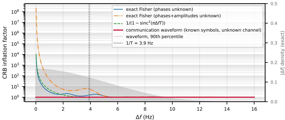
Two-tone frequency CRB inflation (equal powers)
