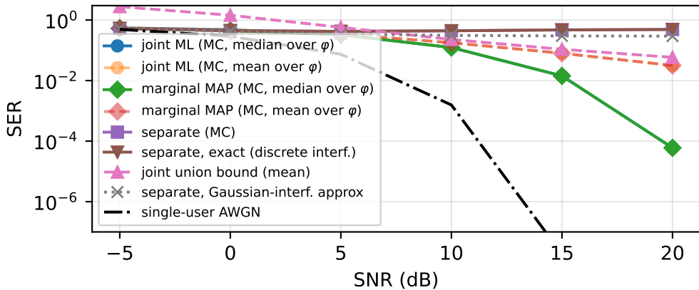
QPSK + QPSK, SIR = 0 dB
