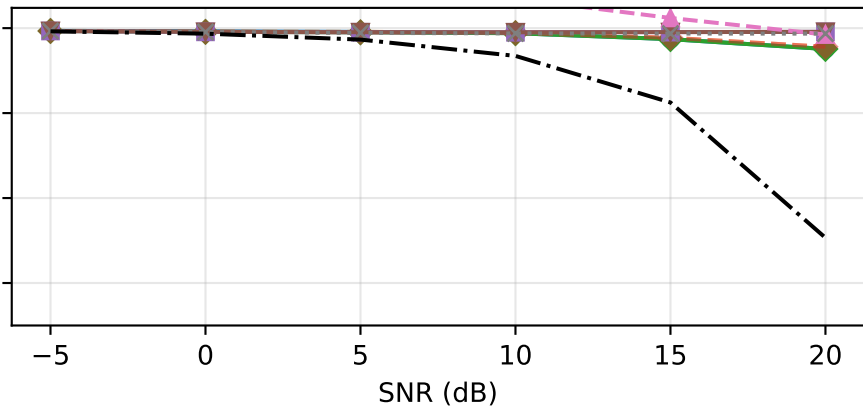
16QAM + 16QAM, SIR = 0 dB
