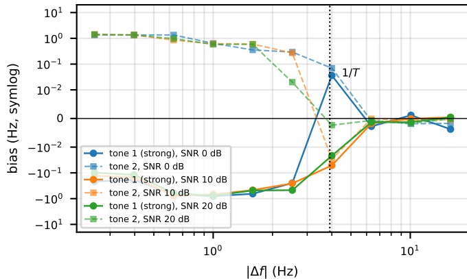
(b) per-tone bias, amplitude ratio 0 dB
