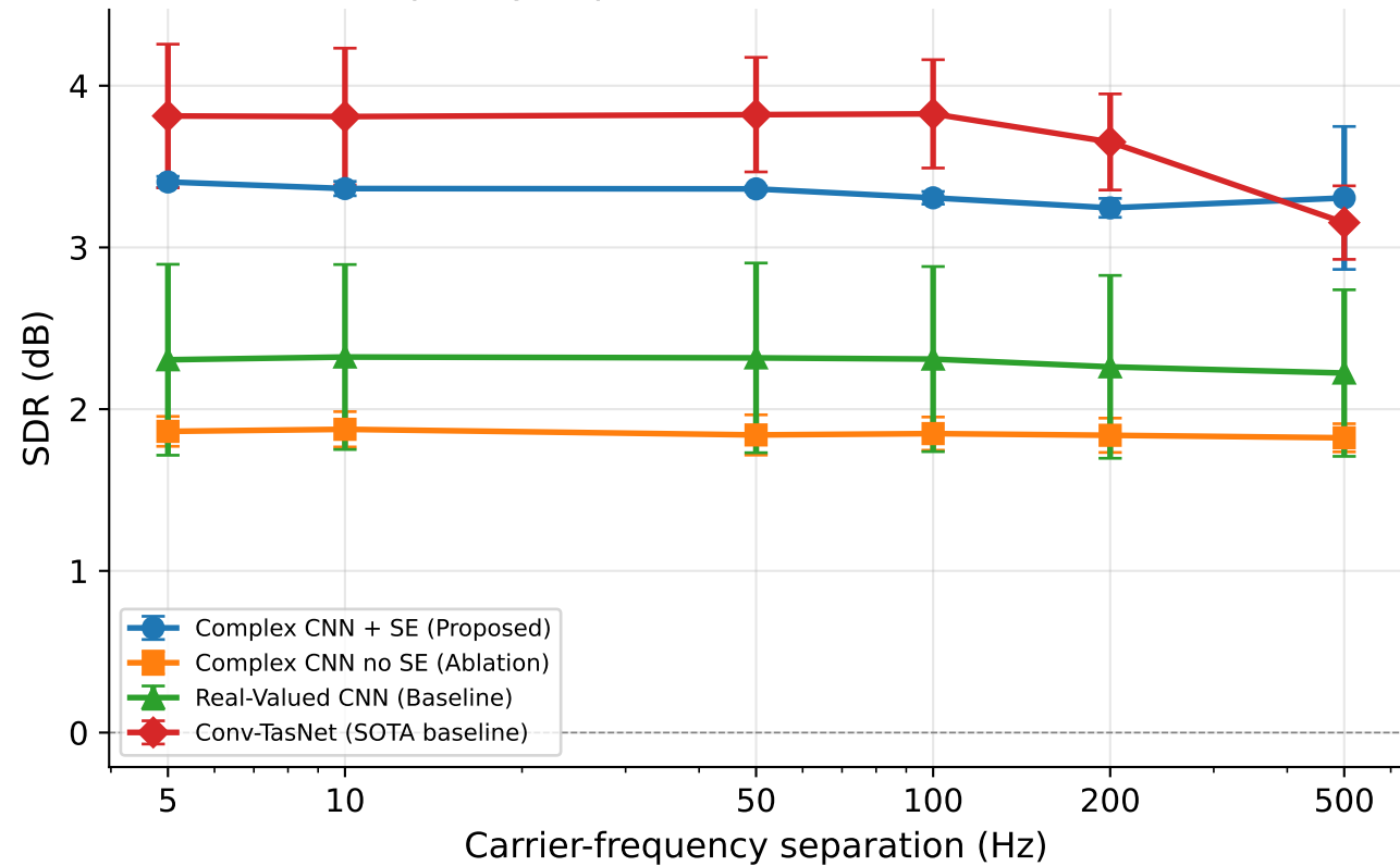
SDR vs Frequency Separation (trained at 5 Hz, mean \pm std)
