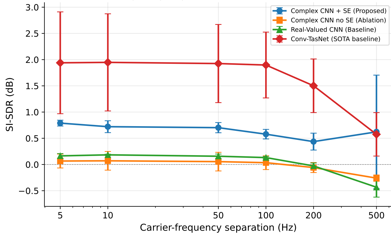
SI-SDR vs Frequency Separation (trained at 5 Hz, mean \pm std)
