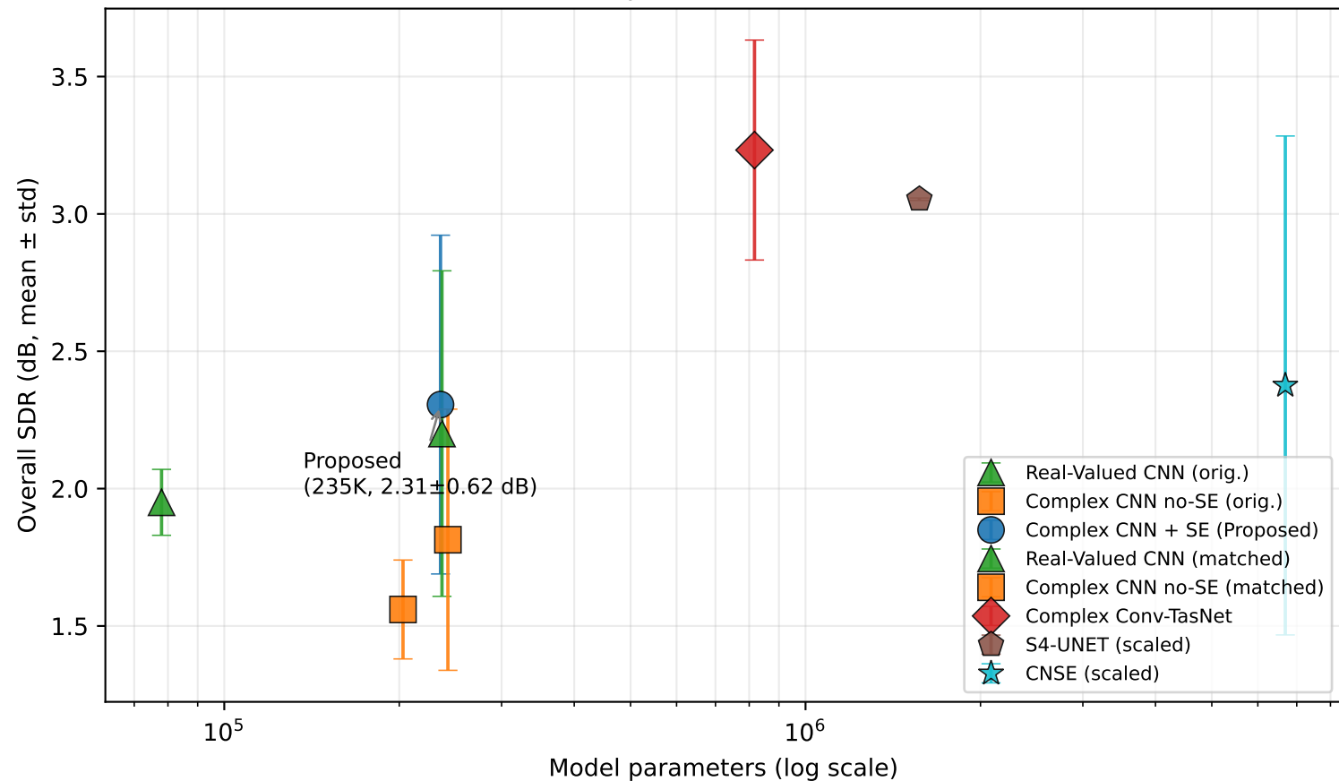
Parameter count vs. SDR performance (5 seeds where available)
