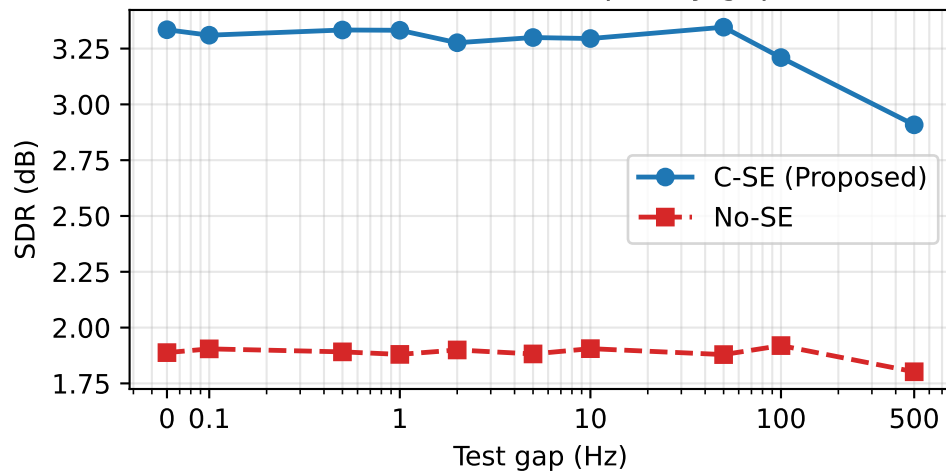
SDR vs. carrier-frequency gap
