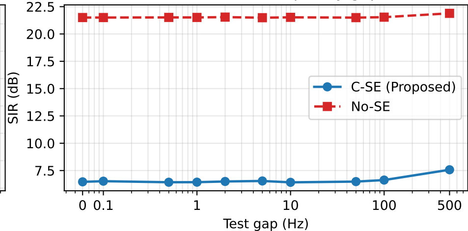
SIR vs. carrier-frequency gap
