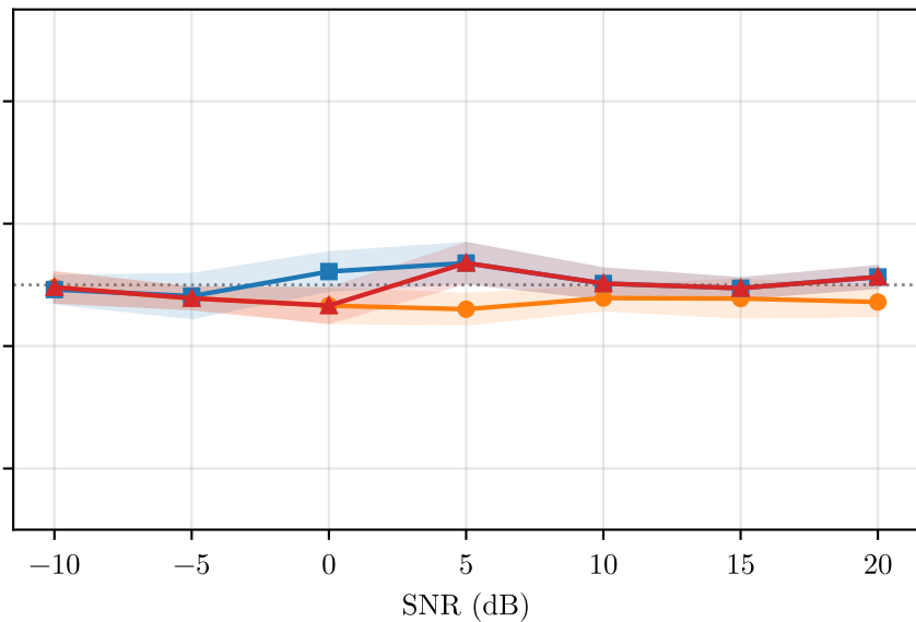
(b) Corrected labels (tile): chance everywhere
