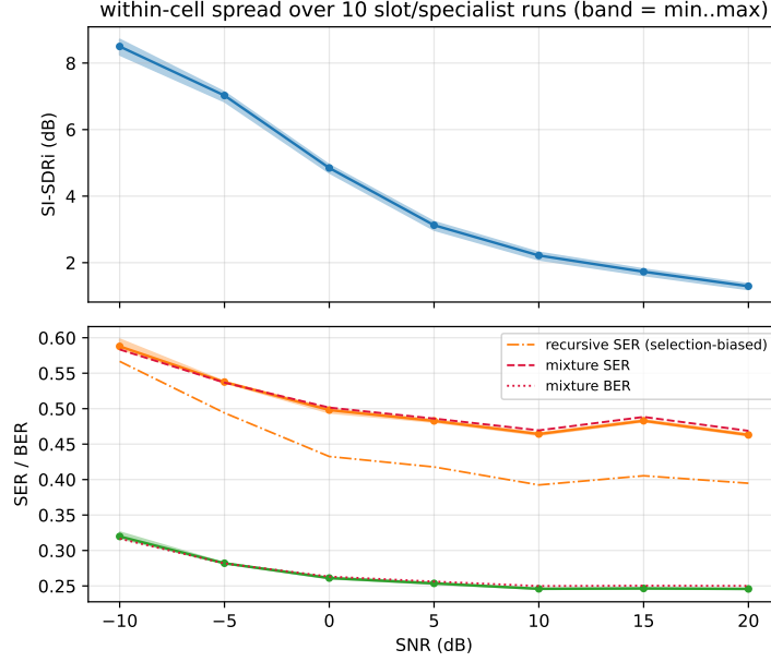
Figure 2: S1: the flat region, per SNR. Top: SI-SDRi of the slot/specialist runs (band = min..max over ten runs). Bottom: compensated SER/BER of the same runs against the mixture baselines (dashed/dotted); the recursive architecture (dash-dot) is shown separately because its miss rate biases its SER downward. Waveform quality improves by 2–8 dB across the grid while bit-level metrics do not move.
