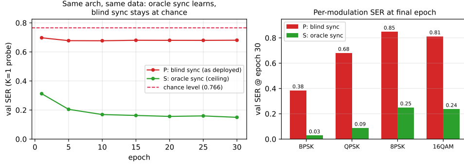
Figure 5: Controlled synchronisation probe ( K=1 , no separation): the same head learns with oracle synchronisation (green, val SER 0.31→0.15) and stalls at chance when synchronising blindly (red). Left: learning curves; right: per-modulation SER at the final epoch.
