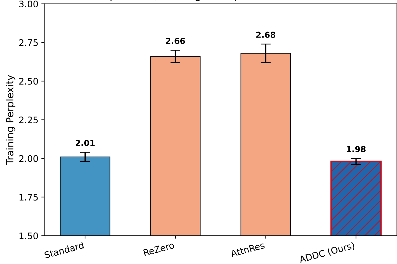
Method Comparison (M config, 25M params, 5k iterations, 3 seeds)
