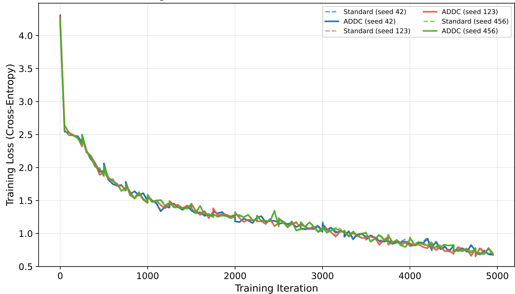
Training Curves: ADDC vs Standard Transformer (3 seeds)
