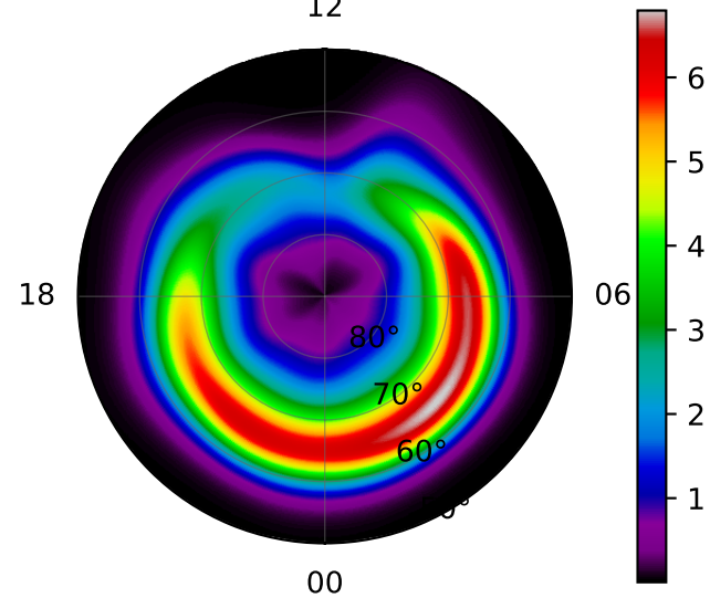
Model E_0 (keV)
