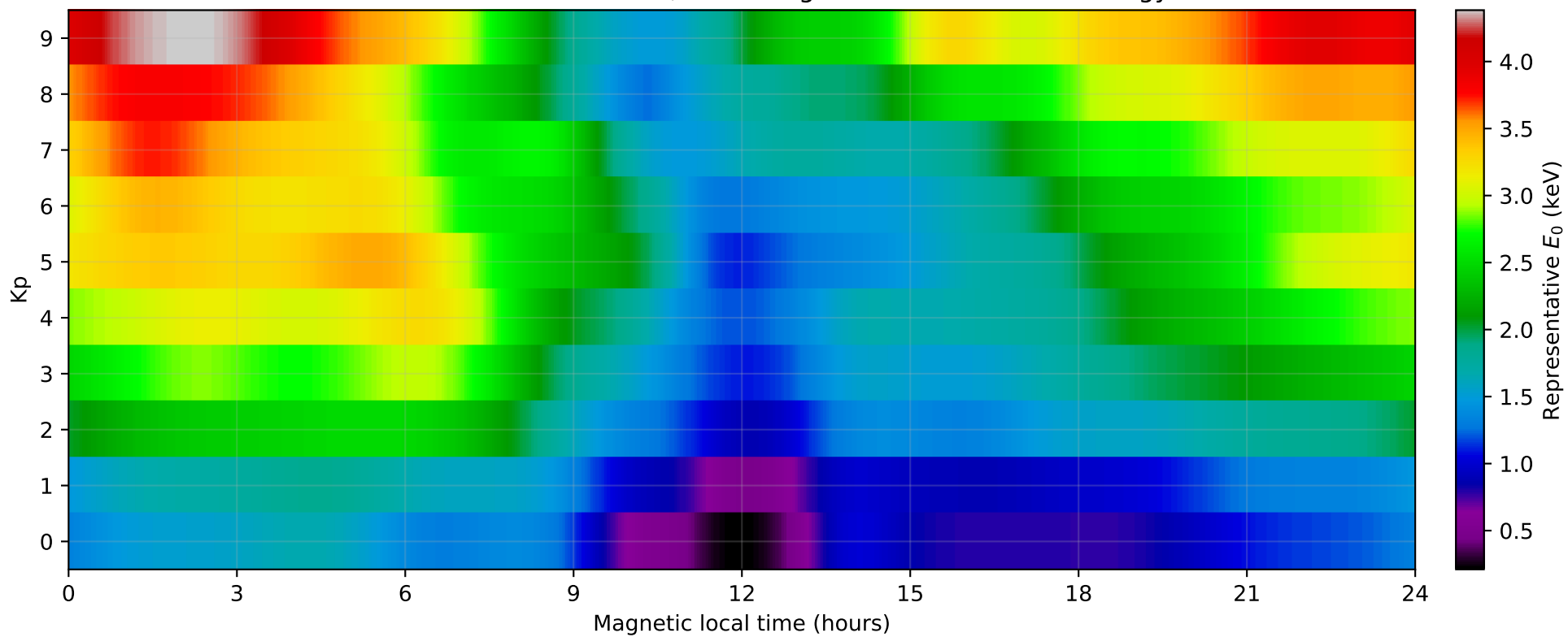
Sensitivity to the definition of the auroral oval
