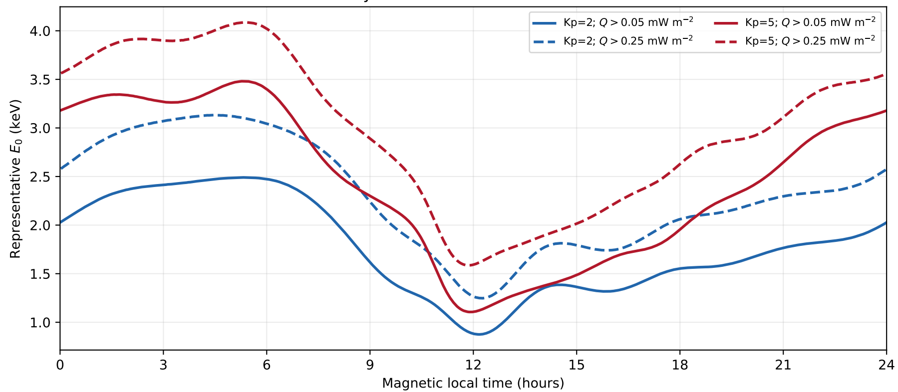
Sensitivity to the definition of the auroral oval
