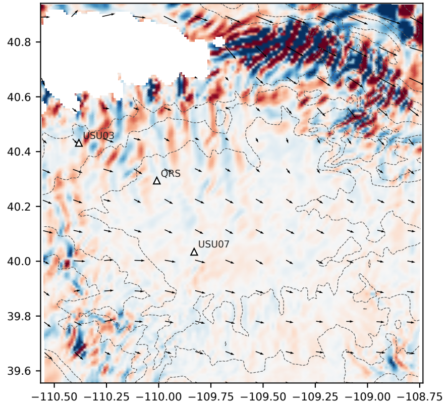
nam_1way_d02 — 02 Feb 14:00 UTC (07:00 MST)
