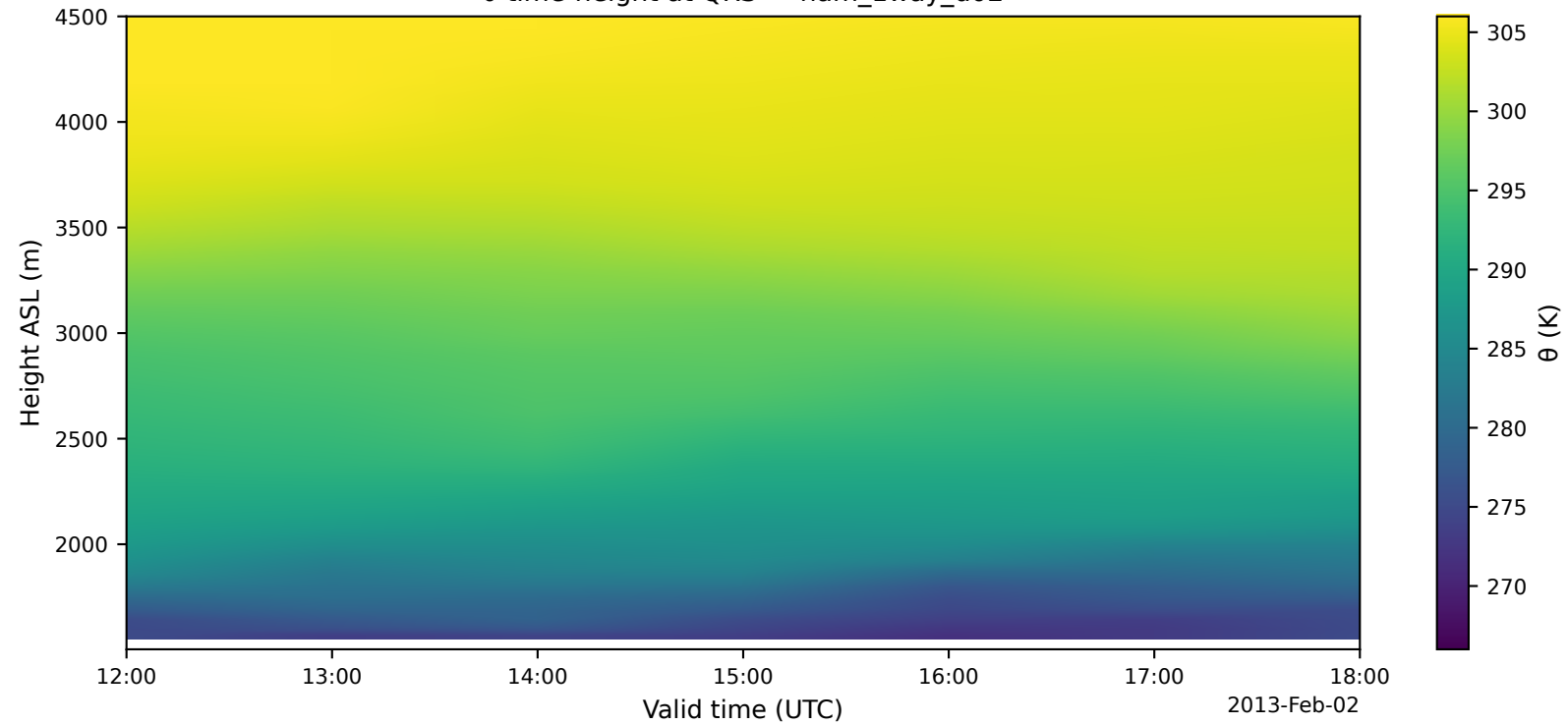
\theta time-height at QRS — nam_1way_d02
