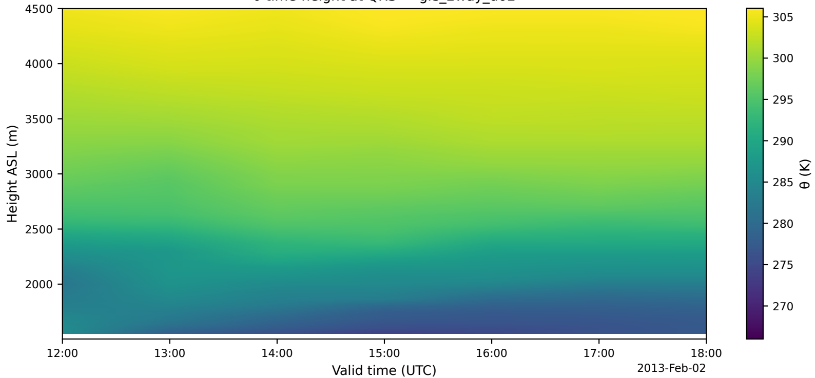
\theta time-height at QRS — gfs_2way_d02
