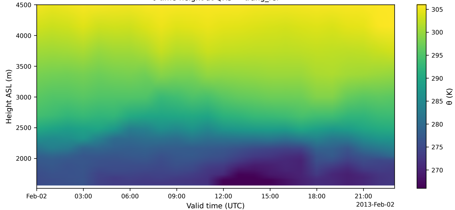
\theta time-height at QRS — trang_ref
