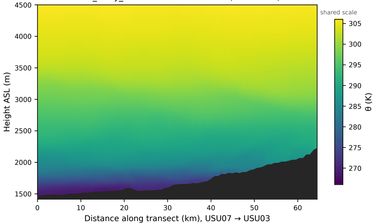
nam_2way_d02 — 02 Feb 16:00 UTC (09:00 MST)
