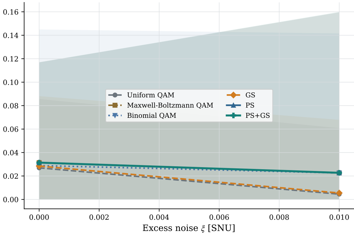
Positive secret-key rate [bit/symbol]
