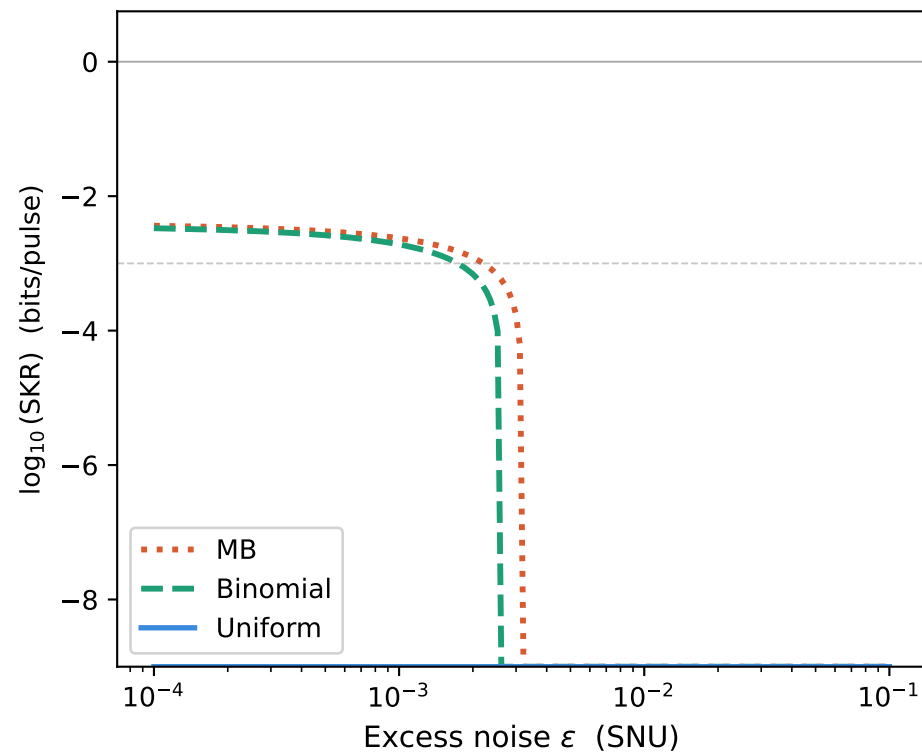
(a) SKR vs Excess Noise
