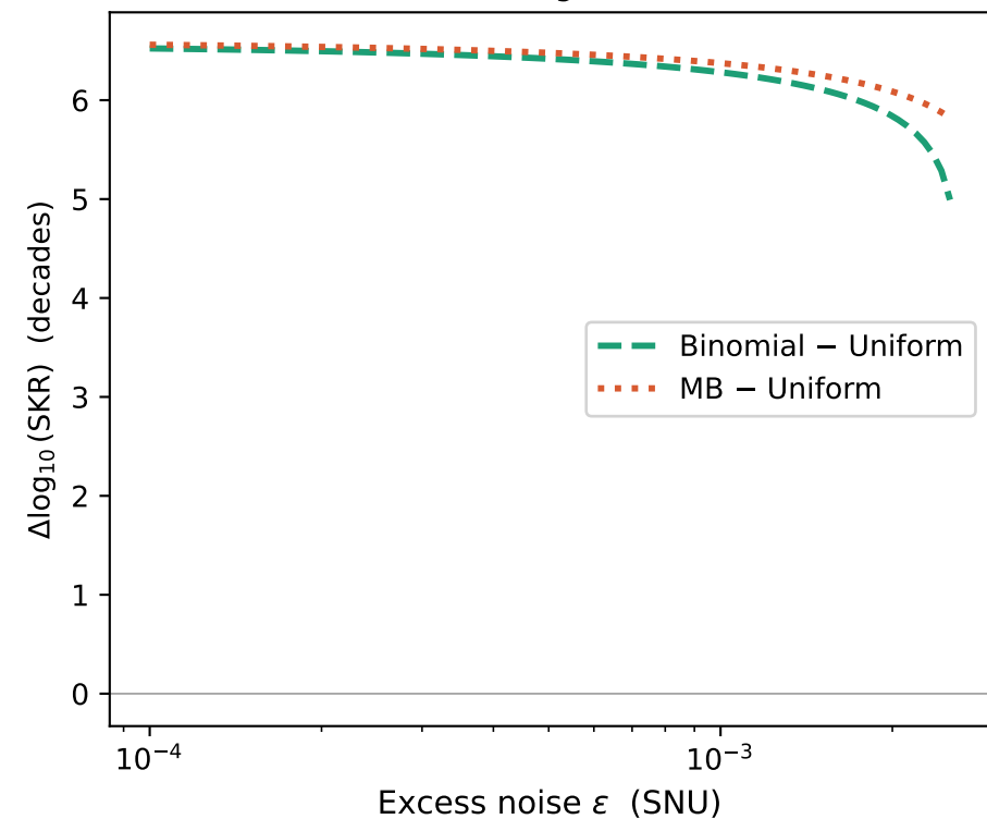
(c) SKR advantage over Uniform
