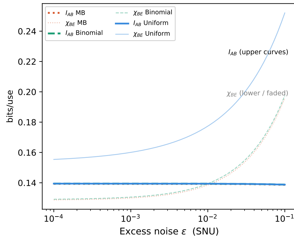
(b) I_{AB} and \chi_{BE} vs Excess Noise
