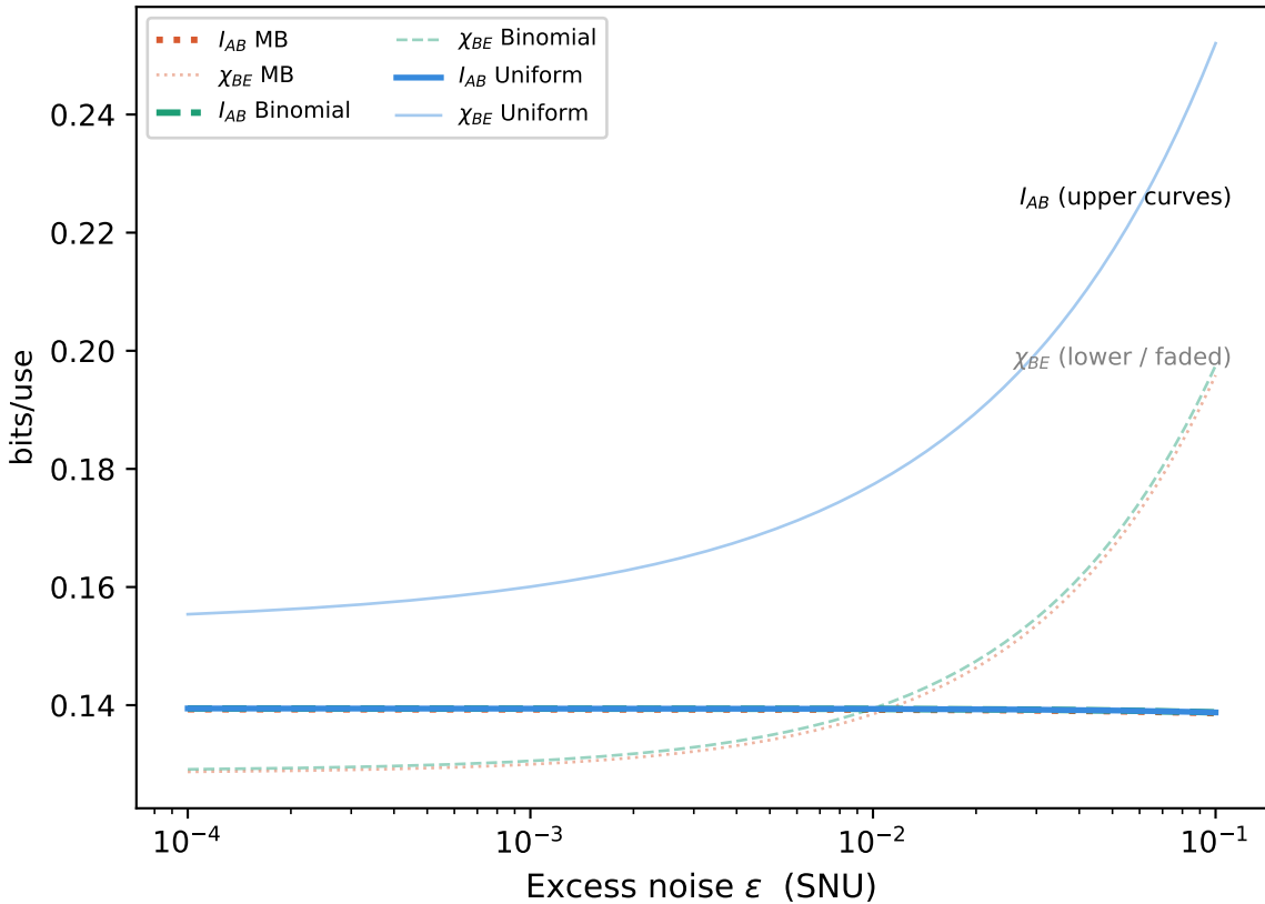
(b) I_{AB} and \chi_{BE} vs Excess Noise
