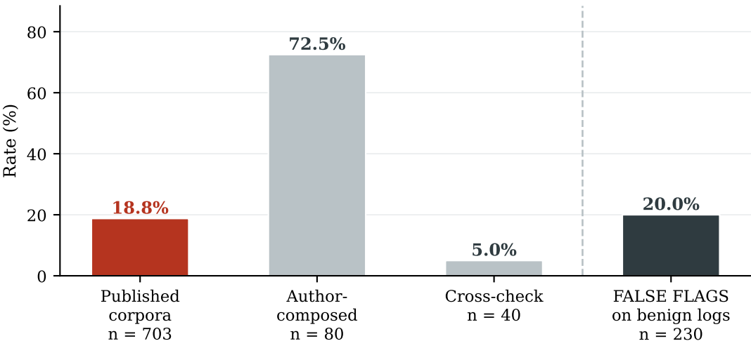
Static pre-filter: block rate by provenance, against its false-flag rate
