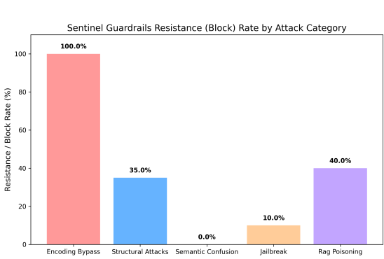
Figure 6. Sentinel guardrails block rate by adversarial attack category. (Source: Author)
