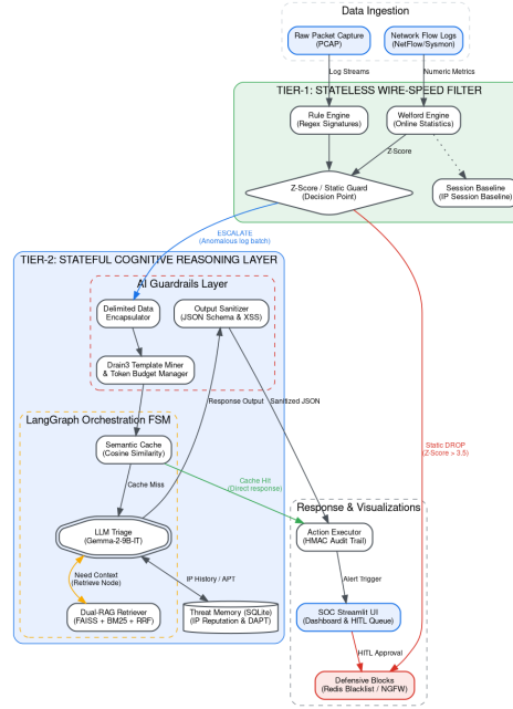
Figure 4. The holistic architecture of the SENTINEL system, illustrating the two-tier data flow and structural components.
