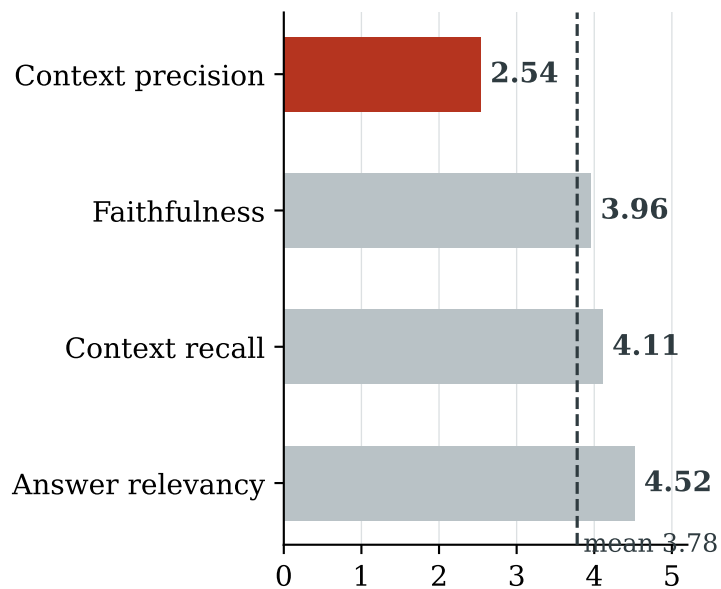
Reasoning quality (judge, 1-5)
