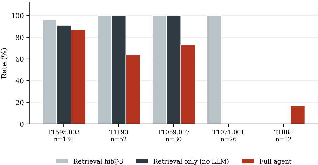
Attribution by technique against the retrieval ceiling
