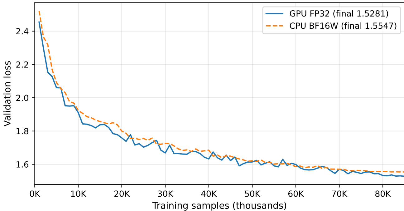
Shakespeare 334K — Validation Loss Curve
