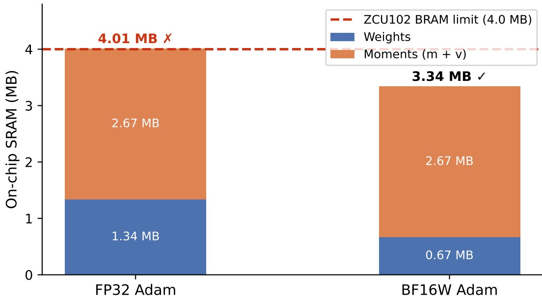
Figure 2: SRAM Budget — NeuronFabric 334K Model (ZCU102 BRAM = 4.0 MB)
