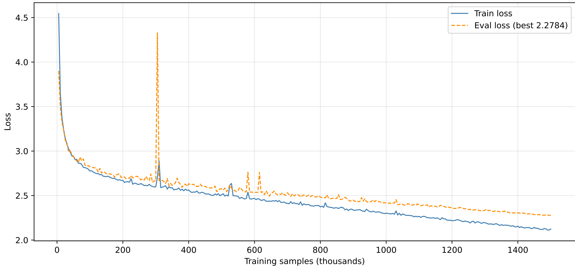
TinyStories 700K — GPU Adam FP32 (1.5M samples)
