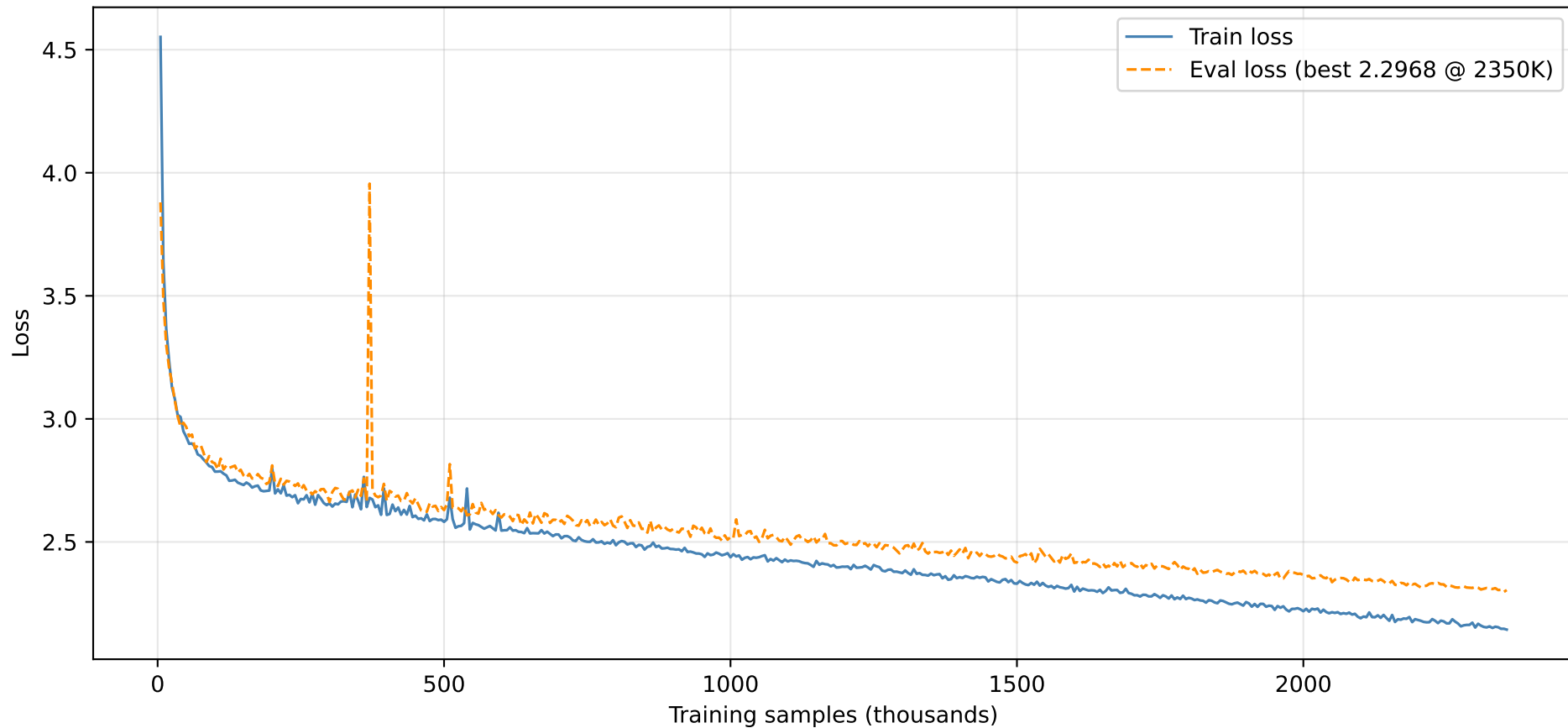
TinyStories 700K — GPU Adam FP32 (up to 2355K samples)
