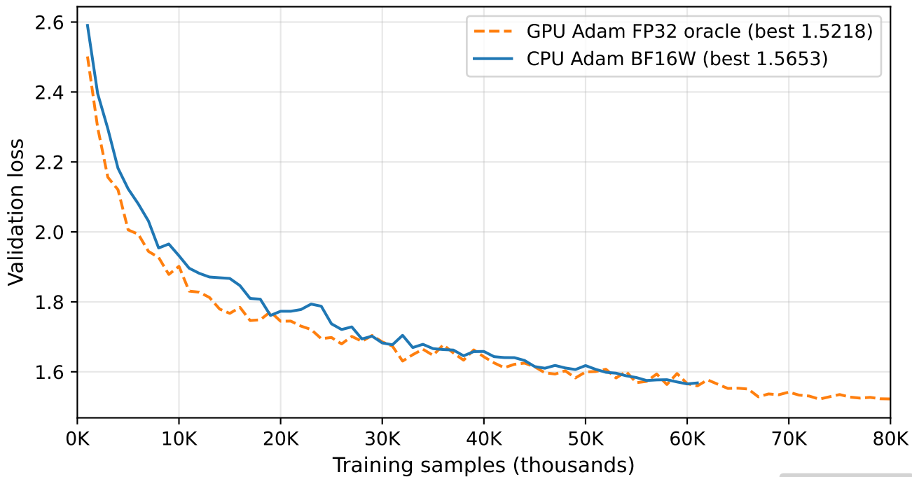
Shakespeare 334K — Validation Loss
