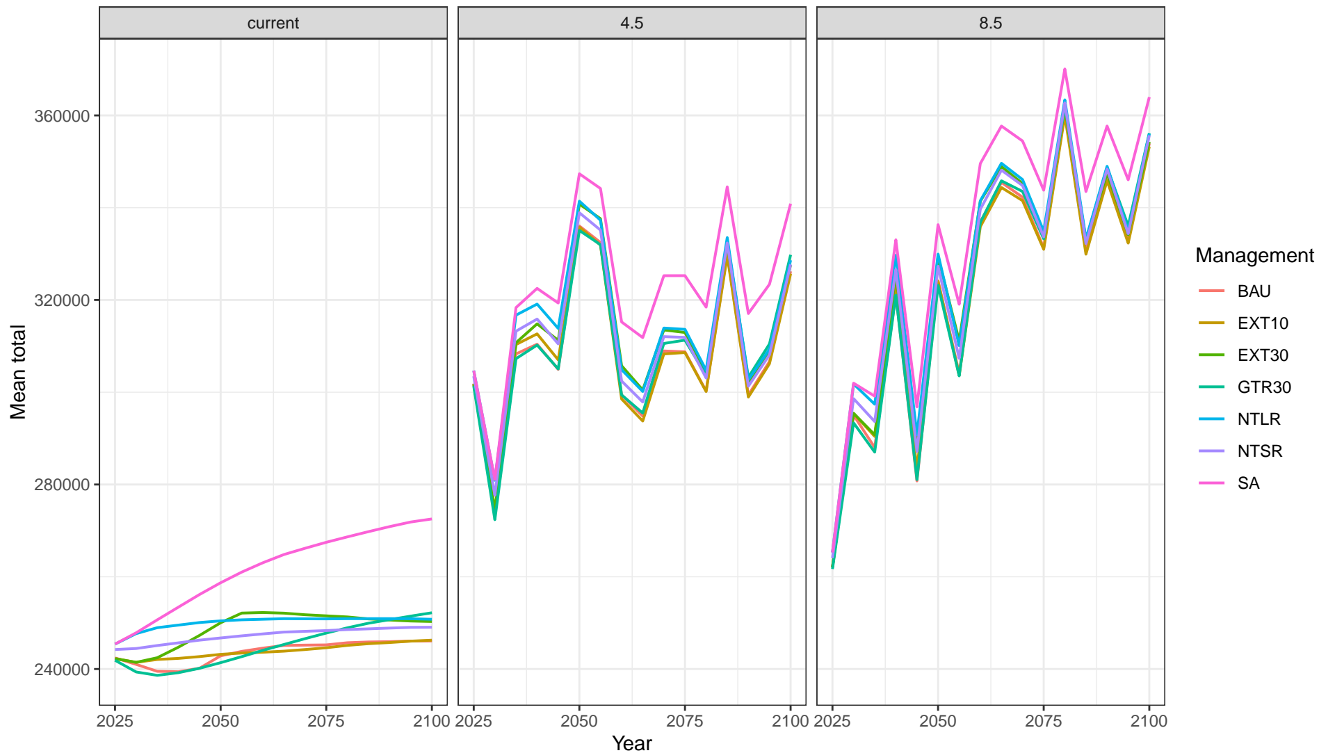
Cluster 2 response to management and climate
