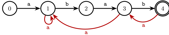
Figure 6.1: The string-matching automaton of P = \text{abab} over \Sigma = \{a, b\} . Forward transitions in black, significant transitions in red; all missing transitions lead to state 0 and are not drawn. There are m = 4 forward and 3 \leq m significant transitions.
