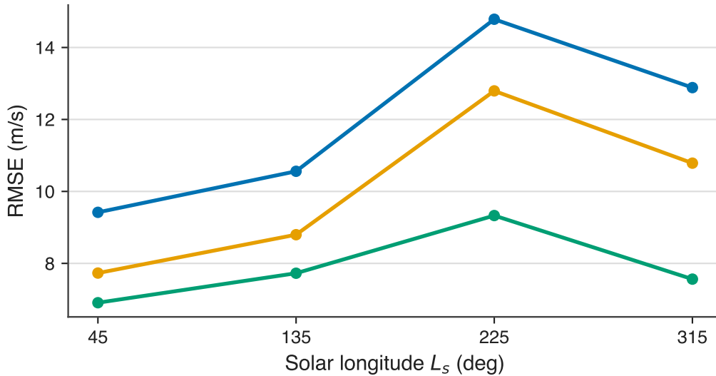
Near-surface wind speed
