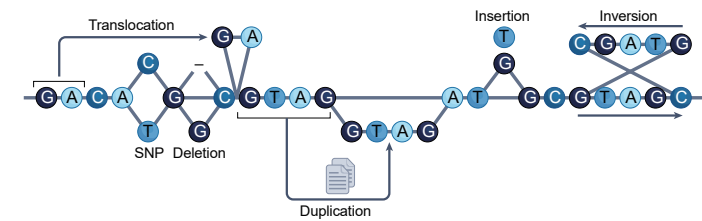
B Structural variation
