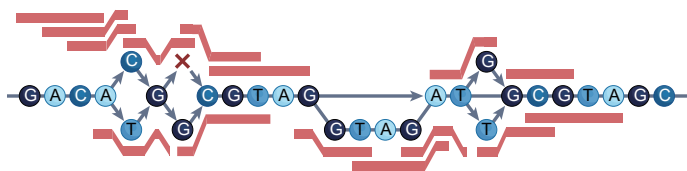
C Short-read alignment to graph
