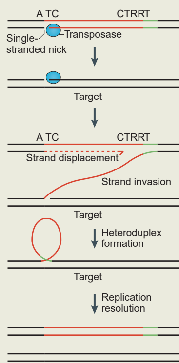
C Helitron
